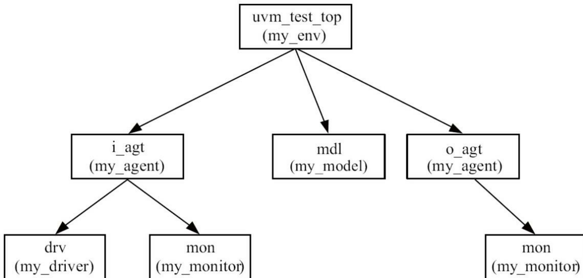
图2-7 UVM树的生长：加入reference model
